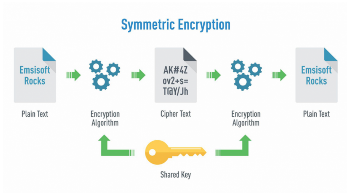
Figure 1: Symmetric Encryption
